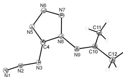
Figure 2. Molecular structure of 2c with thermal ellipsoids set at 30% probability. Selected bond lengths [Å] and angles [°]: C4–N5 = 1.320(1), N5–N6 1.368(1), N6–N7 1.298(1), N7–N8 1.359(1), N8–C4 1.337(1), N8–N9 1.407(1), C4–N3 1.388(1), N3–N2 1.258(1), N2–N1 1.119(1); N5–C4–N8 = 109.80(8), C4–N8–N7 108.08(8), C4–N3–N2 112.89(8), N8–N9–C10 115.84(8); torsion angles [°]: N8–C4–N3–N2 172.77(8), C4–N8–N9–C10 136.88(9).
