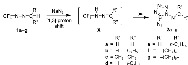
Scheme 2. Synthesis of several 5-azidotetrazoles, 2a–g .
